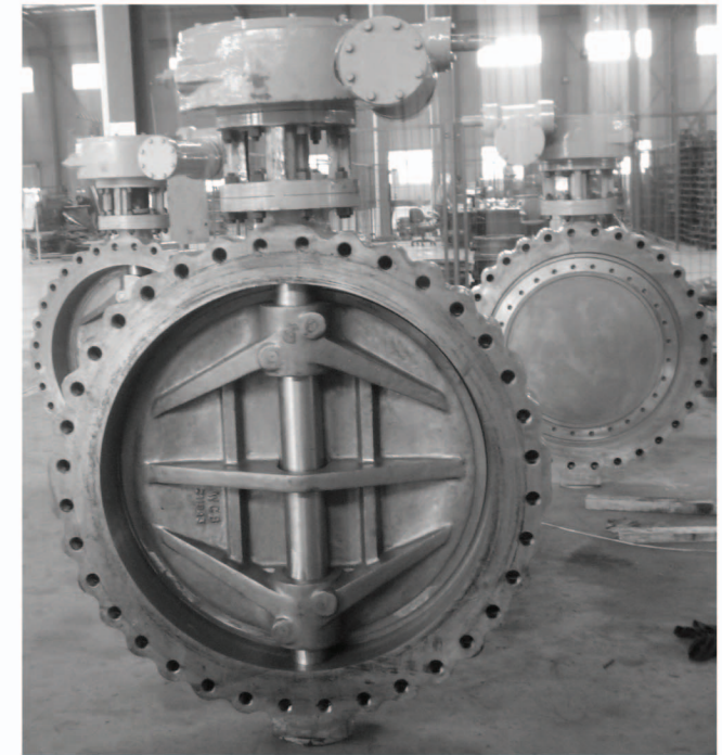
No.3 high performance & double eccentric butterfly valve This valve is disc sealing, more expensive than NO.1 & No.2
